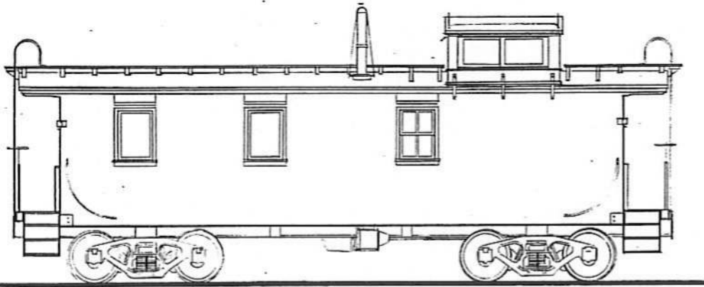
SIDE ELEVATION
